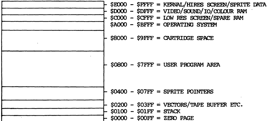
FIGURE 8-2 MEMORY CONFIGURATION AFTER MEM
