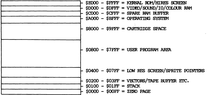
FIGURE 8-1 MEMORY CONFIGURATION BEFORE MEM
